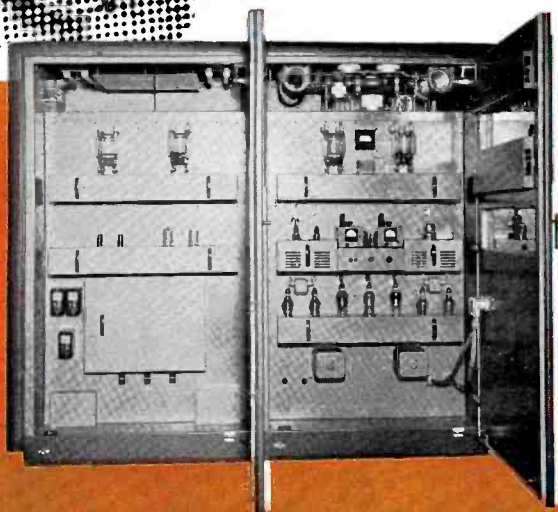
(20T open front view)
